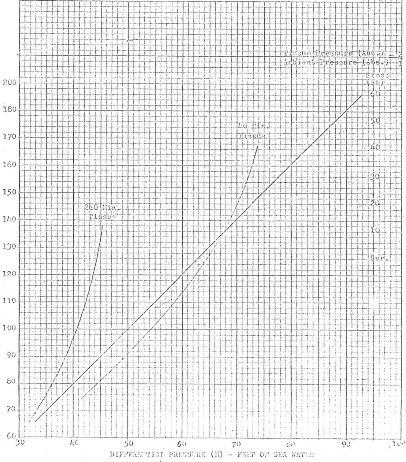
Fig. 12 Maximum allowable final tissue pressure based on allowable differential (E) - 40 and 240 minute tissues related to 2.00:1 ratio of tissue pressure absolute to ambient pressure absolute
